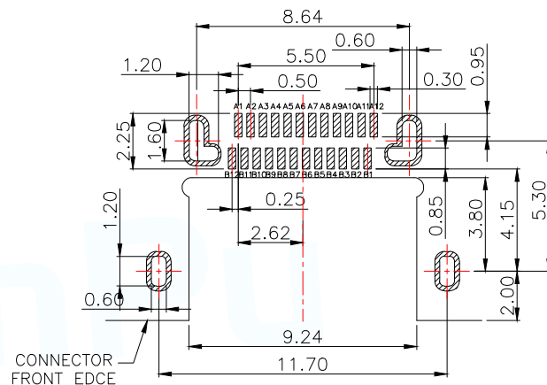
RECOMMENDED PCB LAYOUT(TOP VIEW) THICKNESS 0.60MM;DEFAULT TOLERANCE:±0.05
